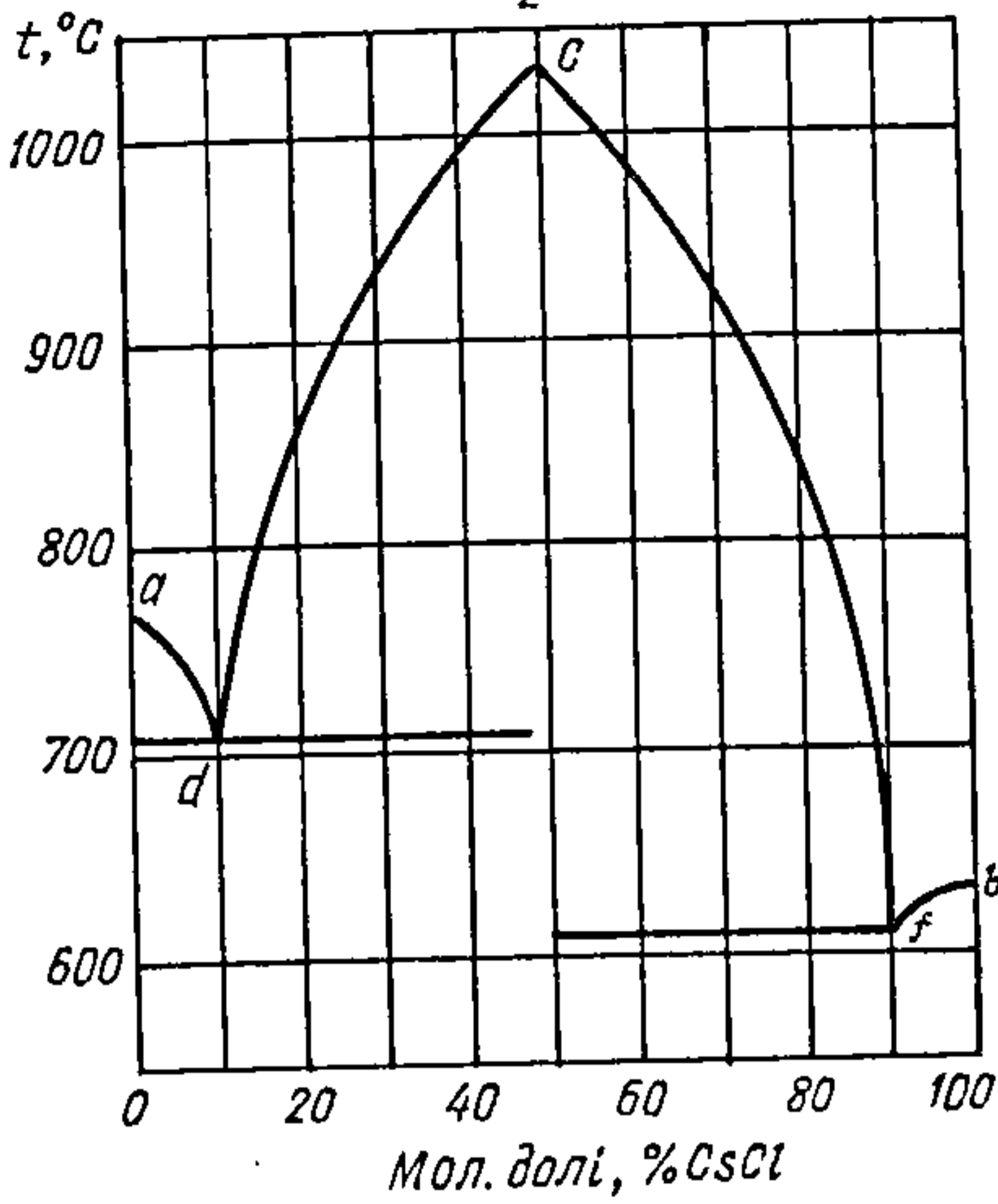
\text{CaCl}_2 - \text{CsCl}
