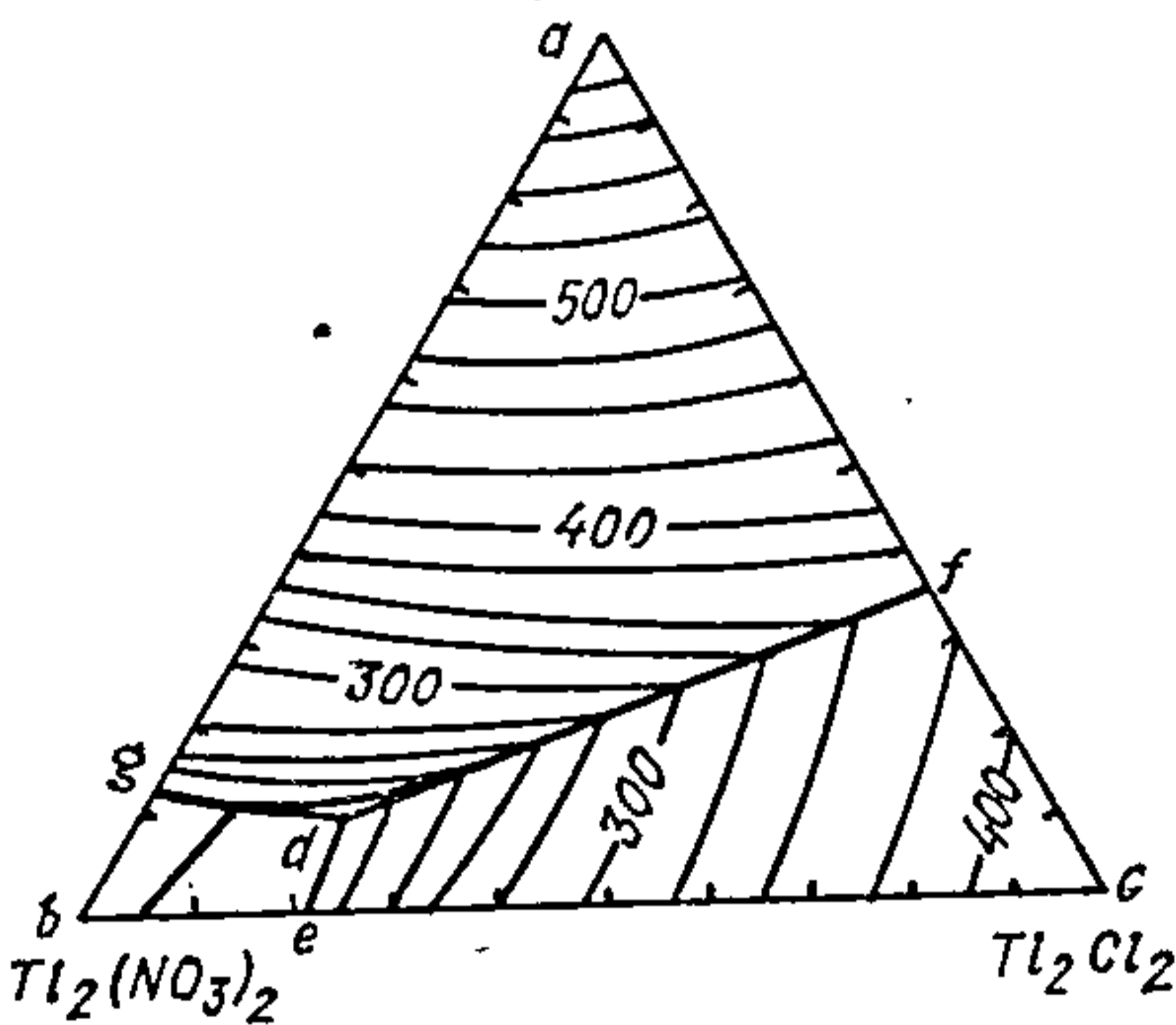
\text{Tl}_2\text{SO}_4 - \text{Tl}_2(\text{NO}_3)_2 - \text{Tl}_2\text{Cl}_2
